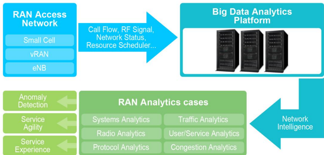
SK Telecom RAN analytics-based intelligent network model
